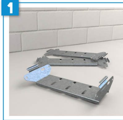
Sin diferencia entre extremos e intermedios. No difference between endings or beginnings.
