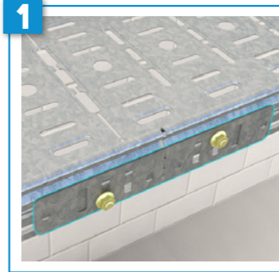
Tramo con tramo. Use the splice plate to join a piece of cable tray with a full cable tray.
